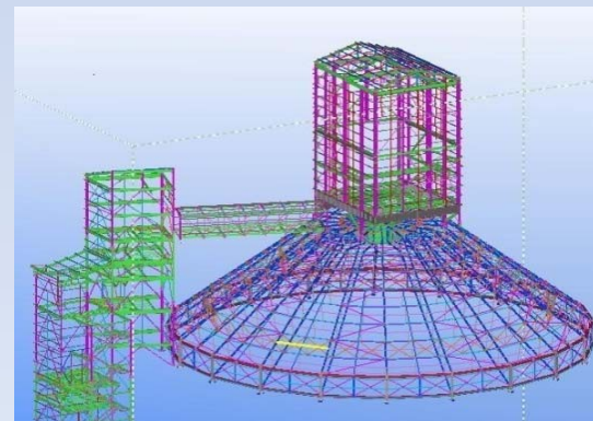
Clinker Dome, Penthouse & CLS
