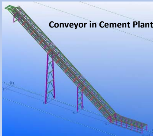
PEB - Structure
