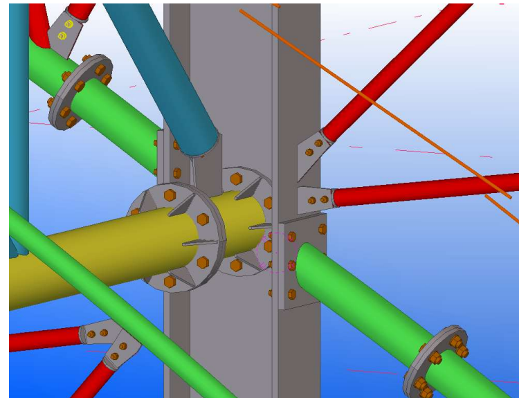
Steel Structure Connection Design
