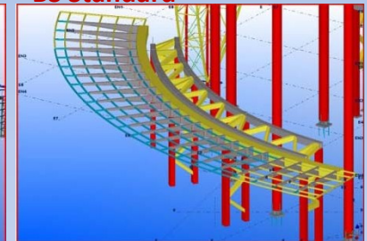
Burj Dubai Hotel Entry Gate BS Standard
